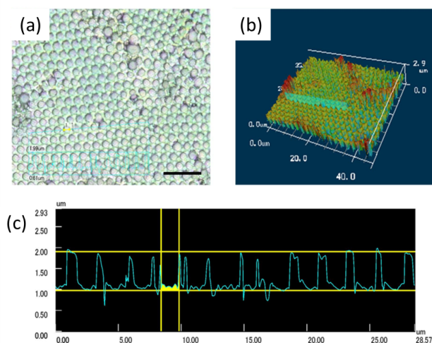
Figure 2. Digital images of the honeycomb film with soybean oil, a) microscope image (Bar= 10μm), b) 3D image, c) cross-section profile.
