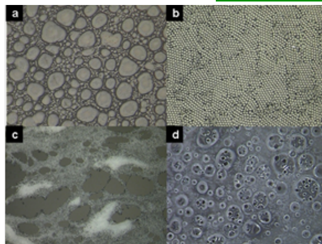
Figure 3. Microscope images of PLLA film by using various solvents a) dichloromethane b) chloroform c) acetonitrile d) THF (×1000).
